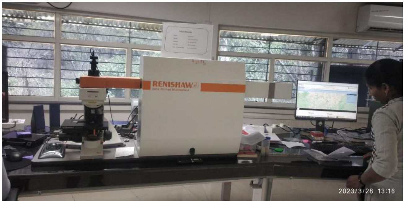
Raman Spectroscope
